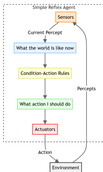
Figure 18.3: Simple Reflex Agent Structure
