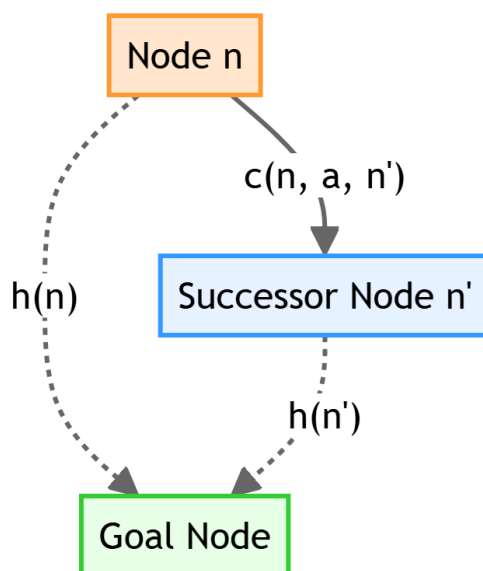
Figure 8.1: Heuristic Consistency Inequality Triangle
