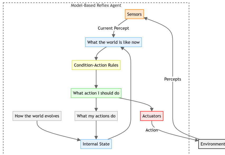
Figure 18.4: Model-Based Reflex Agent Structure
