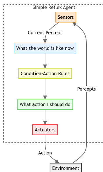
Figure 4.2: Simple Reflex Agent Structure
