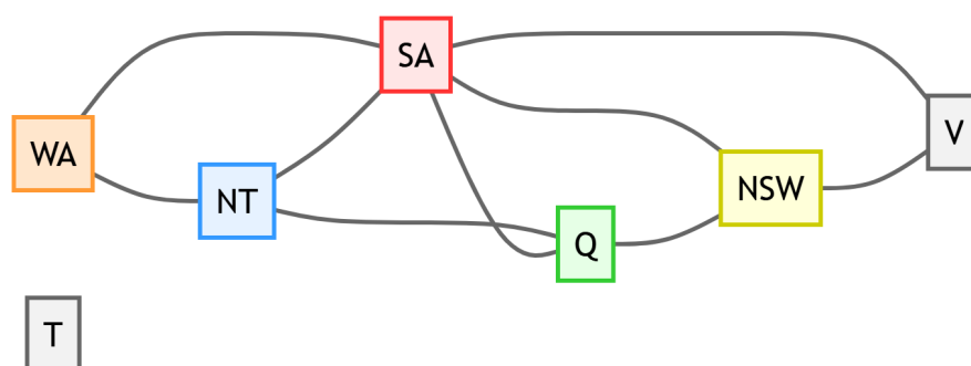
Figure 18.9: Australia Map-Coloring Outline
