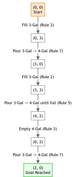
Figure 6.2: Water Jug Traced Solution Path
