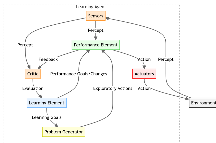
Figure 4.6: Learning Agent Structure
