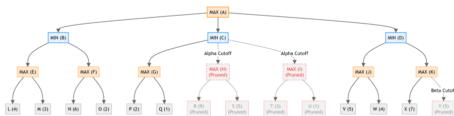
Figure 18.10: Alpha-Beta Pruning Game Tree
