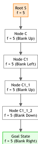
Figure 8.3: 8-Puzzle State Transition Trace
