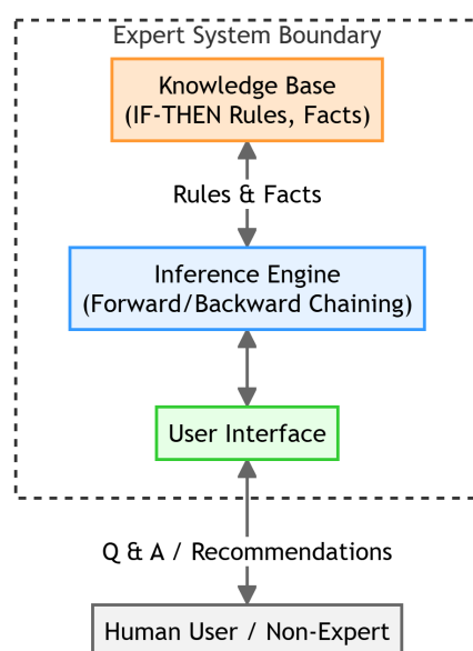
Figure 18.2: Expert System Architecture
