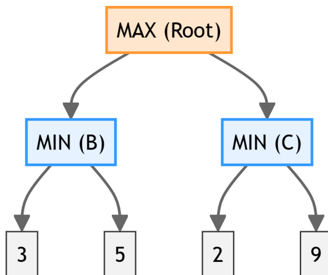
Figure 12.1: Minimax Game Tree
