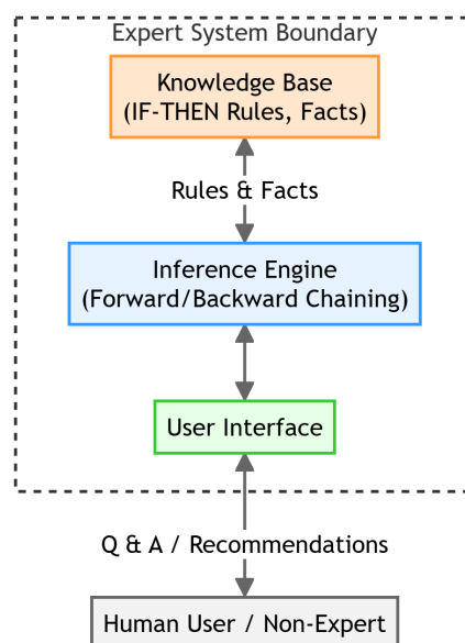
Figure 2.4: Expert System Architecture
