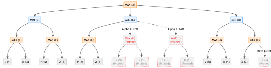
Figure 12.2: Alpha-Beta Pruning Game Tree
