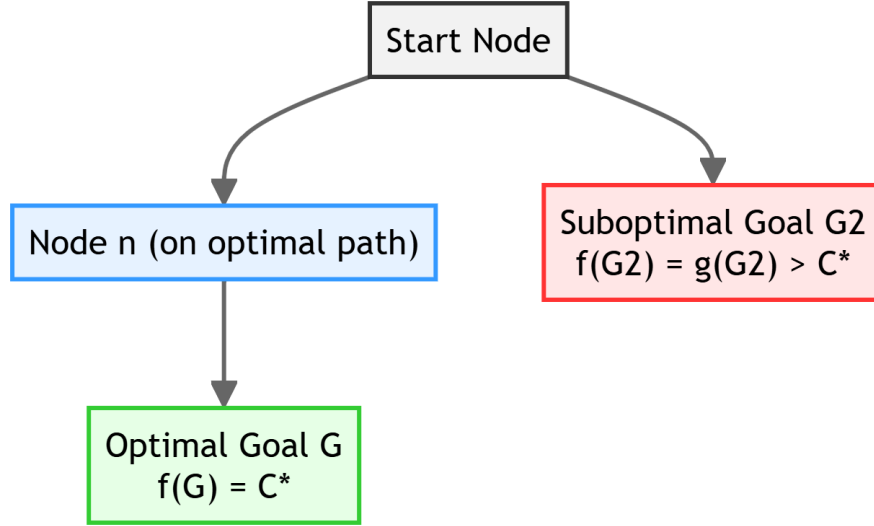
Figure 8.2: A* Optimality Contradiction Tree
