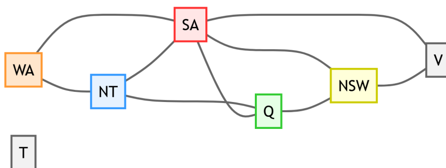
Figure 10.1: Australia Map-Coloring Outline
