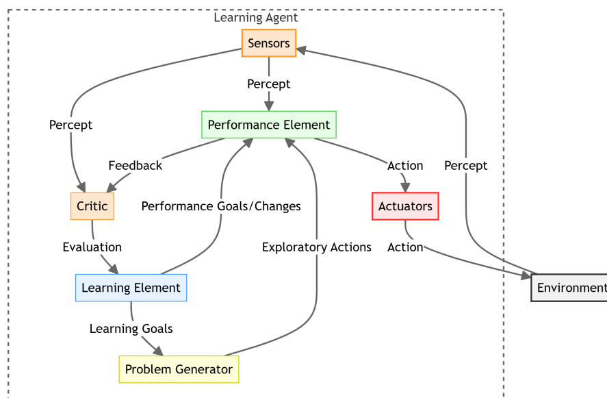
Figure 18.5: Learning Agent Structure
