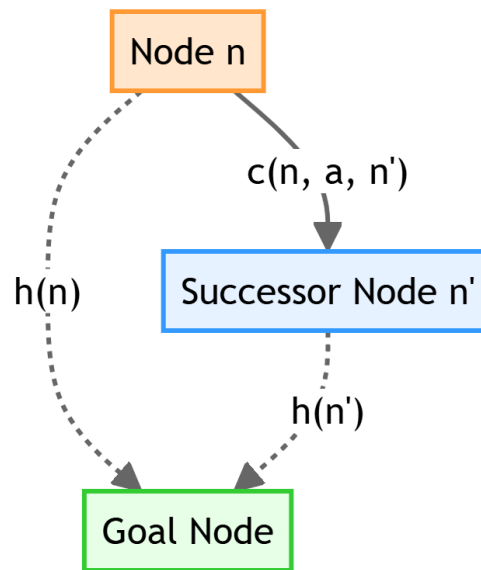
Figure 18.7: Heuristic Consistency Inequality Triangle
