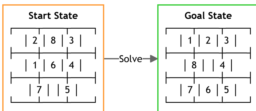
Figure 6.1: 8-Puzzle Start and Goal States
