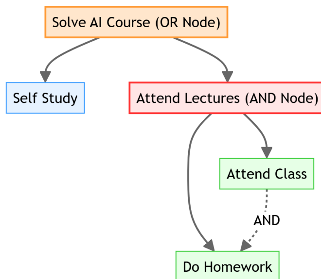
Figure 8.4: AND-OR Graph Decompositions
