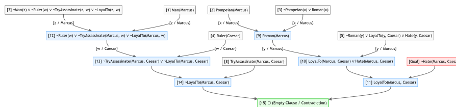
Figure 18.13: Resolution Refutation Proof Tree
