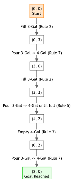
Figure 18.6: Water Jug Traced Solution Path
