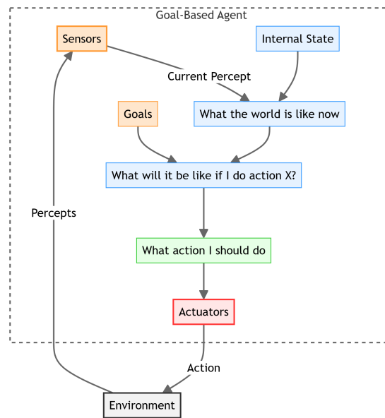
Figure 4.4: Goal-Based Agent Structure
