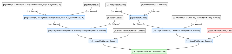
Figure 16.1: Resolution Refutation Proof Tree
