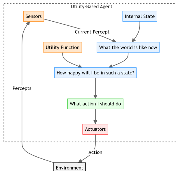
Figure 4.5: Utility-Based Agent Structure
