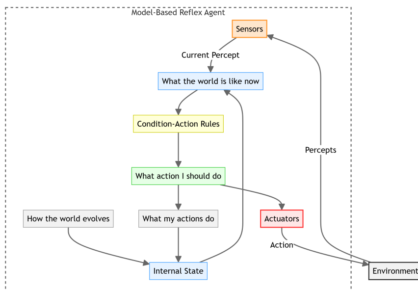
Figure 4.3: Model-Based Reflex Agent Structure
